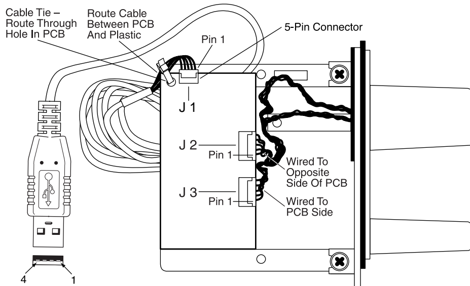
Figure 2-1. Cabling
