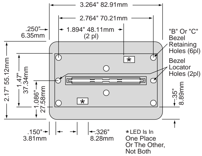
Figure B-1. Bezel "A" Dimensions
