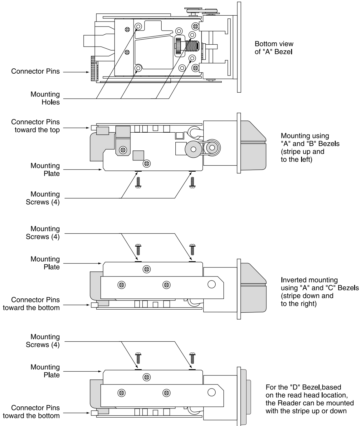
Figure 2-9. Mounting Configurations
