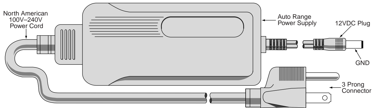
Figure 2-13. Power Supply
