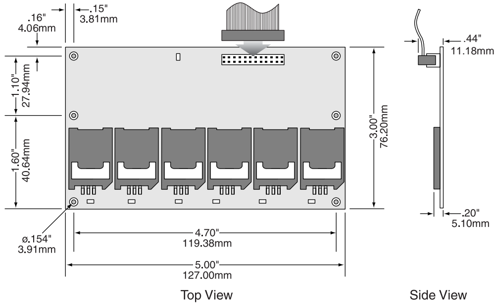
Figure A-3. SAM Ranch Dimensions
